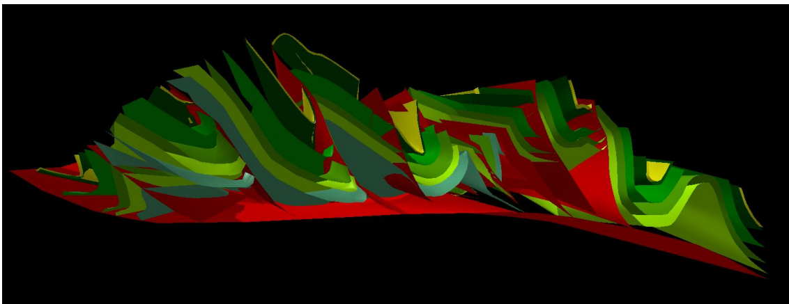
Fig. 1. Lateral view of the 3-D model, showing the present days fold-and-thrusts structures.
