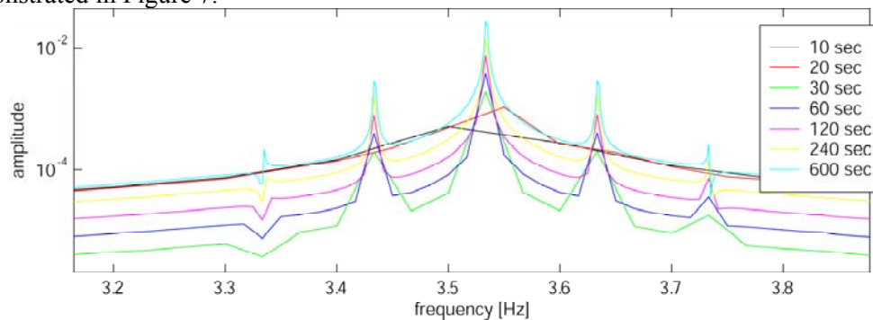
Figure 7: Development of the spectrum of nonlinear oscillations in a spherical pore during 600 s for filling level z_0 = 0.9 of the pore liquid. The frequency spacing of the multiple peaks is a typical feature of nonlinear systems and corresponds to the frequency of the driving oscillation at 0.1 Hz. Natural oscillation frequency of pore: \nu = 3.527 Hz, mass of liquid in pore m = 2.64 \cdot 10^{-5} kg.
