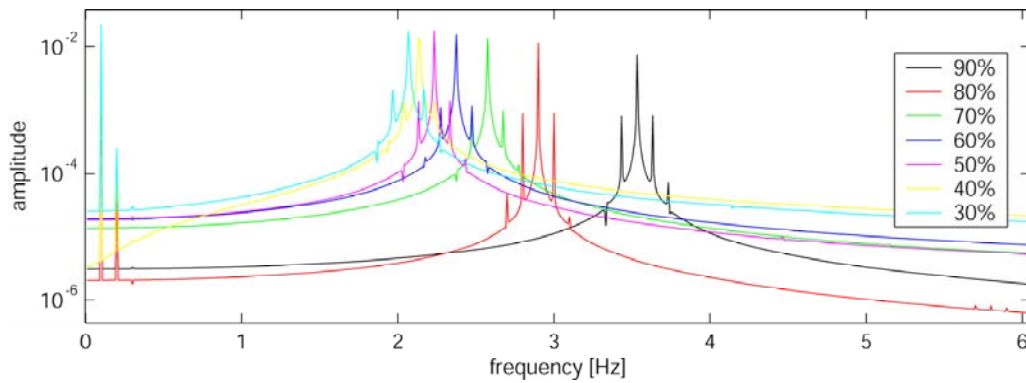
Figure 6: Spectrum of nonlinear oscillations in a spherical pore for different filling levels z_0 between 0.3 and 0.9 of the pore liquid. The frequency spacing of the multiple peaks is a typical feature of nonlinear systems and corresponds to the frequency of the driving oscillation at 0.1 Hz, which also produces its own overtone at 0.2 Hz. For demonstration reasons, the damping was set to zero which leads to sharper peaks.
