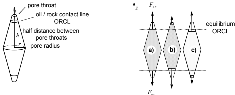
Figure 3: Schematic representation of a simple bi-conical pore geometry which enables low frequency oscillations of the contained liquid along the z-direction. The liquid surface boundary forms the oil/rock contact line (ORCL) between the oil and water phases as well as the water wetted pore surface where capillary forces occur. a) liquid in equilibrium: the capillary forces F_{+z} in positive and F_{-z} in negative z direction balance each other; b) Situation after a small displacement of the liquid in the positive z-direction: F_{+z} has decreased and F_{-z} has increased compared to the equilibrium. The resulting restoring force drives the liquid back along the negative z-direction towards its equilibrium position; c) same as b) with dislocation in the negative z-direction.
