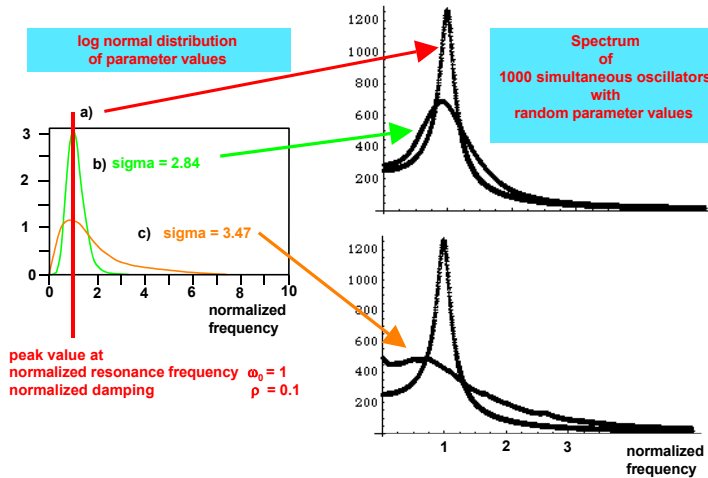
Figure 4: Numerical simulation of the superimposed spectrum of 1000 linear harmonic oscillators for three different parameter distributions: a) all oscillators with normalized resonance frequency at \omega_0=1 and damping \rho=0.1 ; b) both resonance frequency and damping vary according to a log-normal distribution with \sigma = 2.84 ; c) both resonance frequency and damping vary according to a broad log-normal distribution with \sigma = 3.47 .
