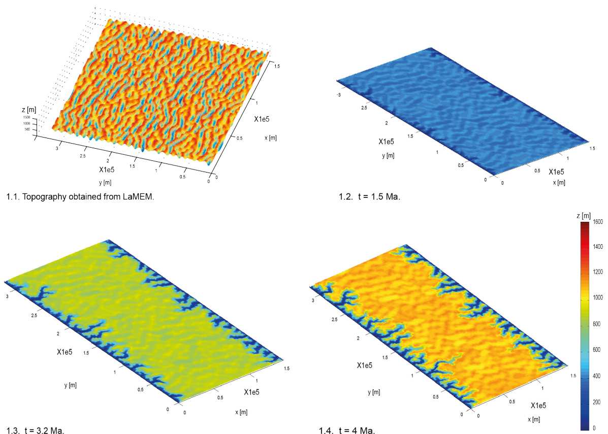
Figure 1: Landscape evolution through time (numerical parameters: number of elements: 32962, number of nodes: 16698).
